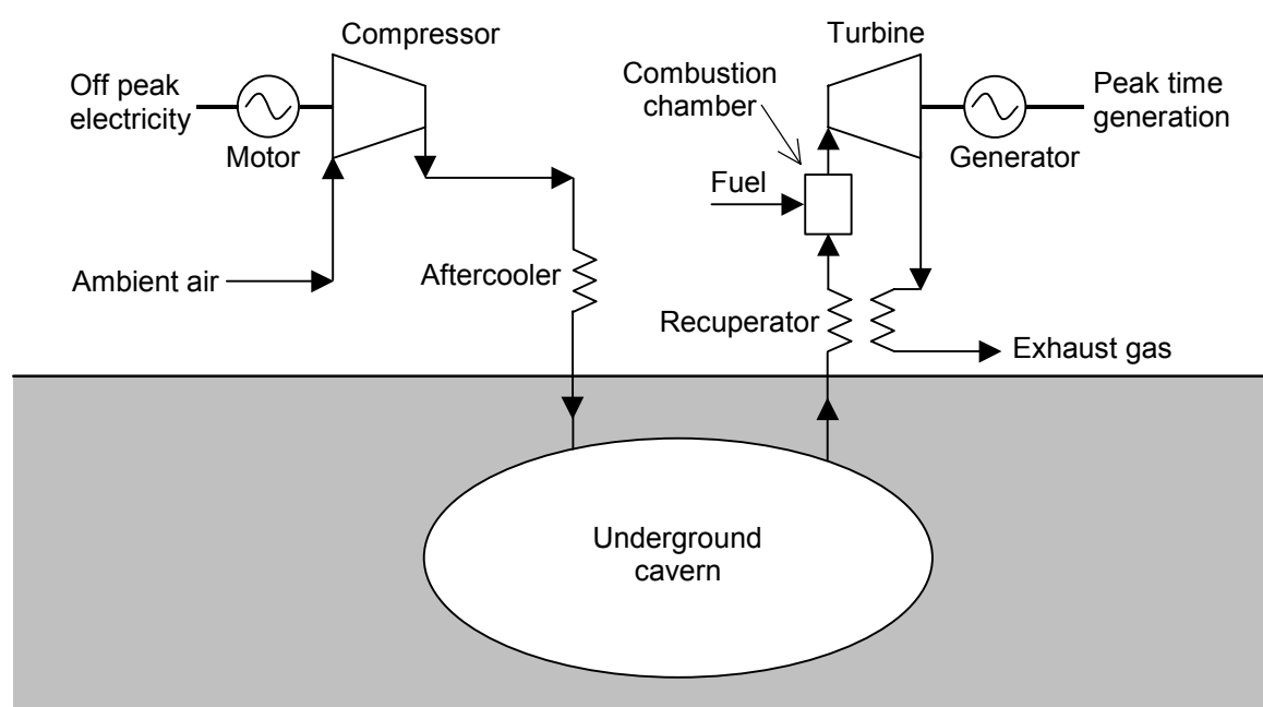
Figure 2.1 Schematic of a Compressed Air Energy Storage System
