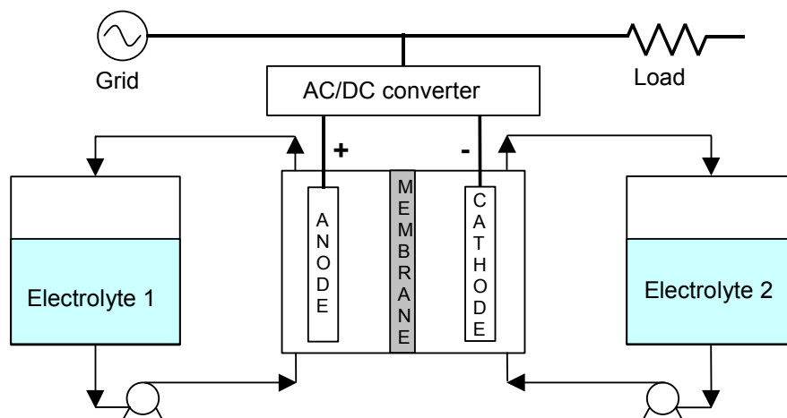
Figure 4.1 Schematic of a Redox Flow Cell Energy Storage System
