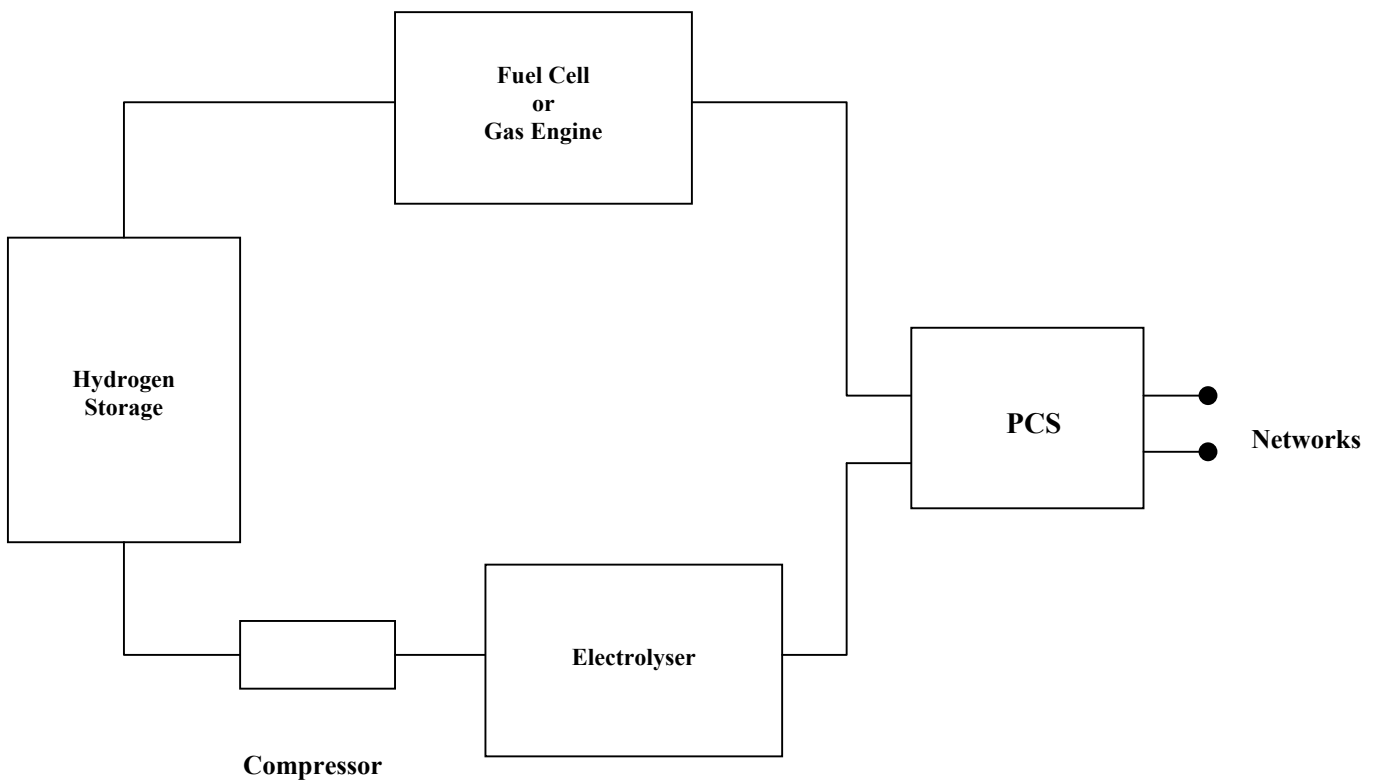
Figure 6.1 Diagrammatic Representation of Hydrogen Energy Storage System
