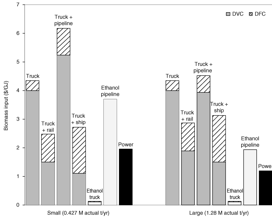
Fig. 4. Woodchip transportation costs for biomass and products more than 500 km.
